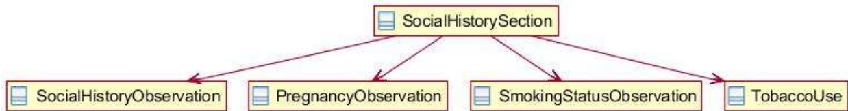
Figure 147: Social history section UML diagram
