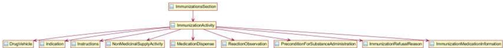
Figure 257: Functional Status section UML diagram (larger copy)
