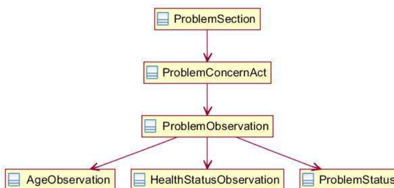
Figure 130: Problem section UML diagram
