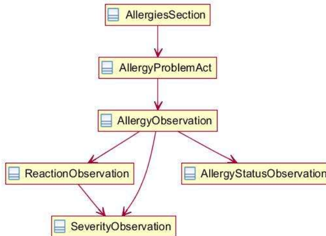
Figure 79: Allergies section UML diagram
