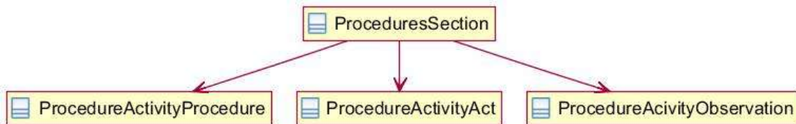
Figure 140: Procedures section UML diagram
